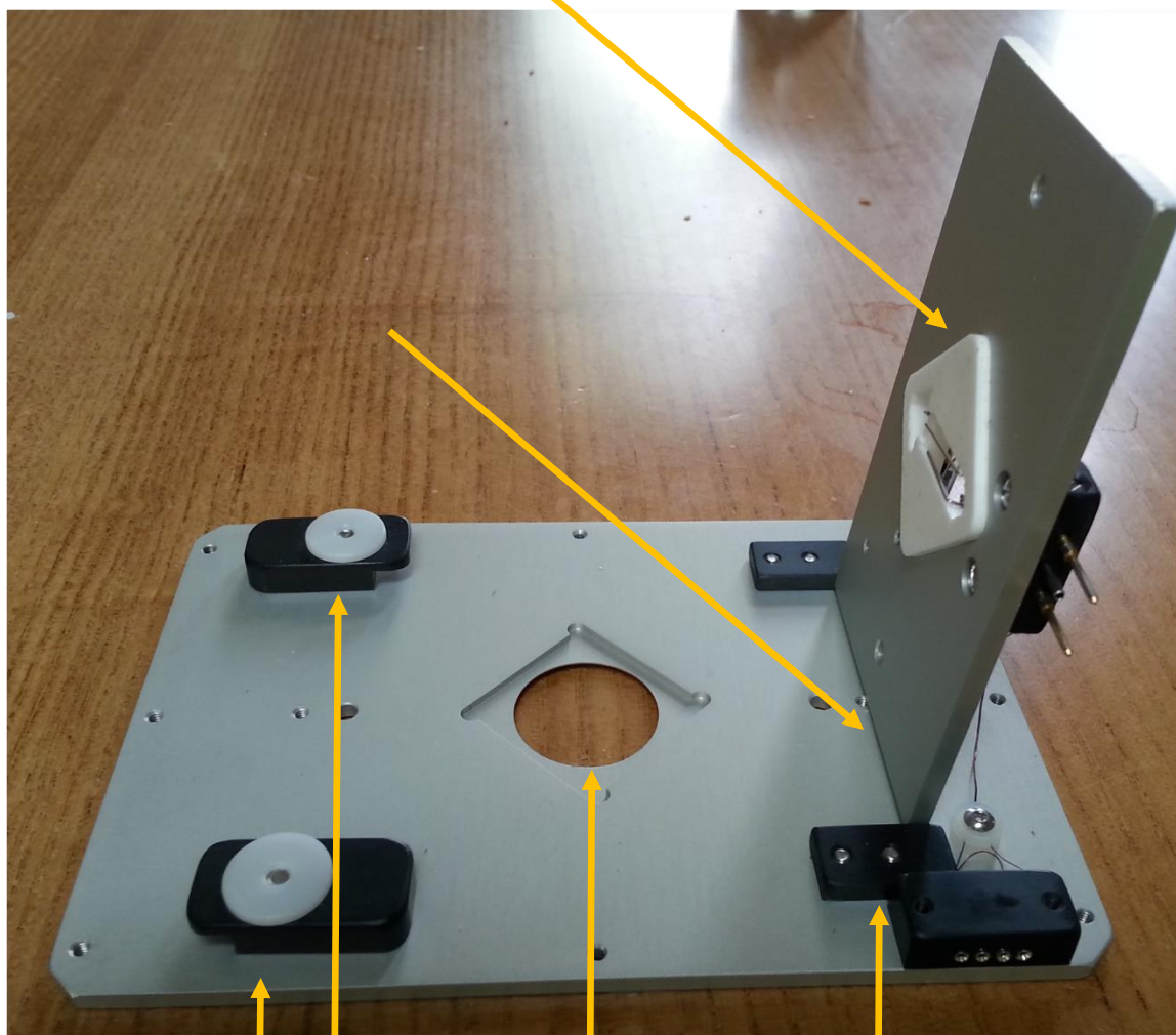
Well for 25 mm cover glass
